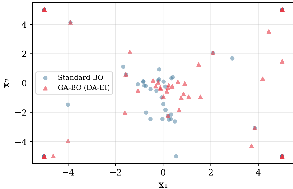
Evaluated Points (dim 1-2) - Ackley-5D
