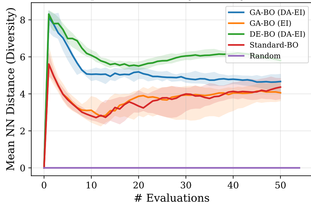
Population Diversity - Ackley-5D
